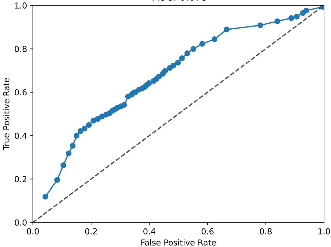
RORA_RORB ROC Curve AUC: 0.673
