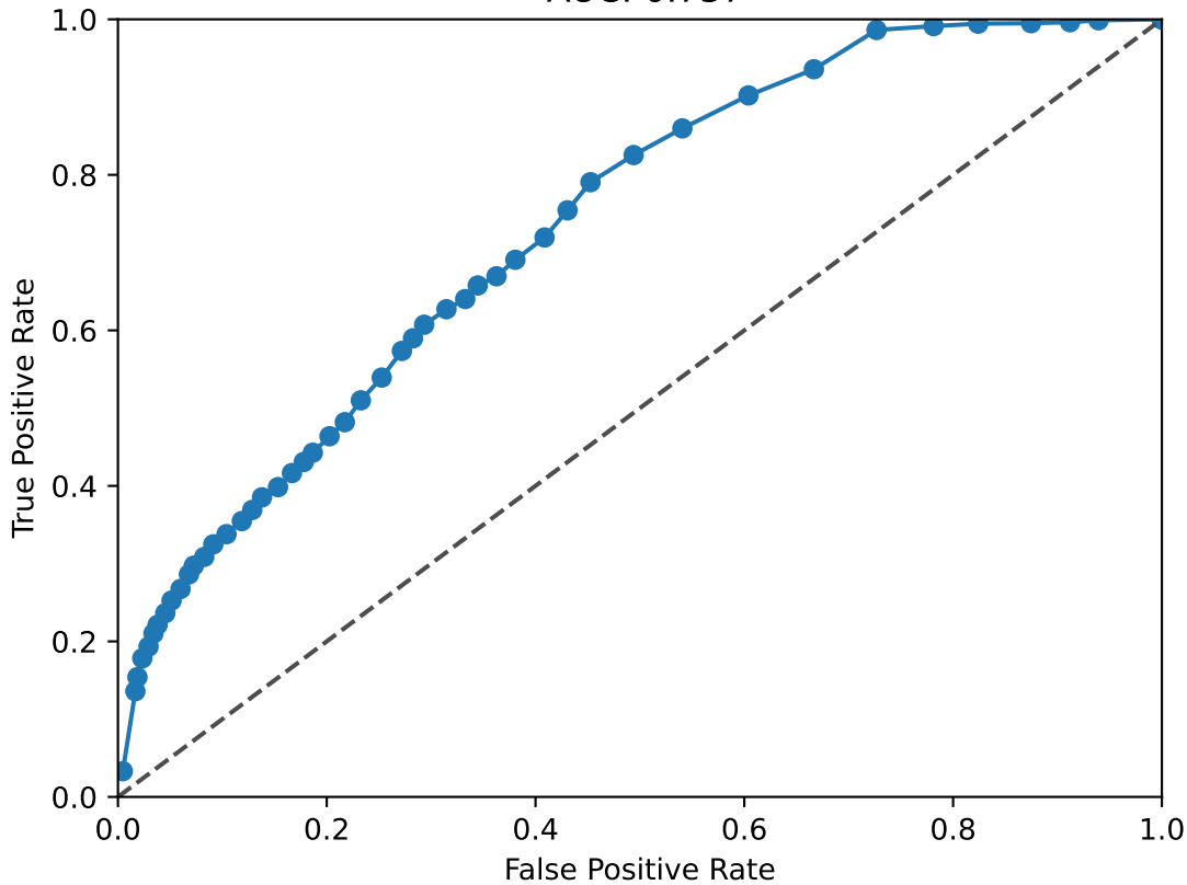
RUNX1 ROC Curve AUC: 0.737
