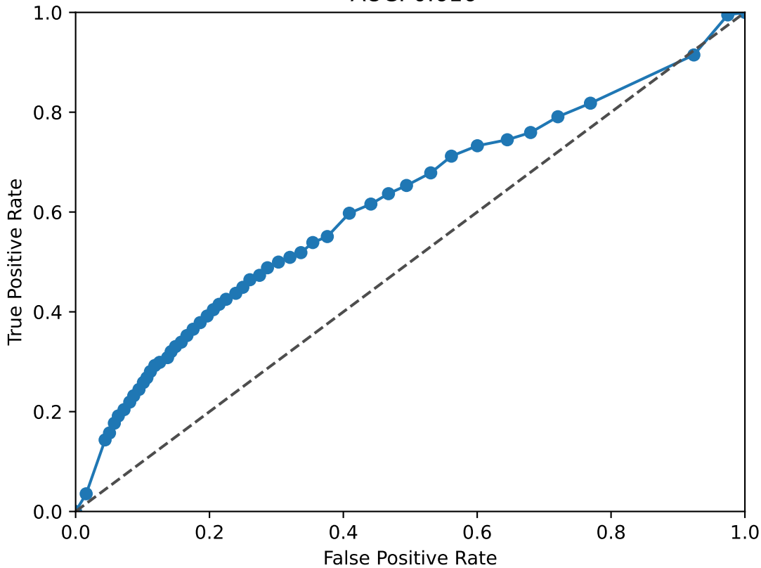
SIX1 ROC Curve AUC: 0.616
