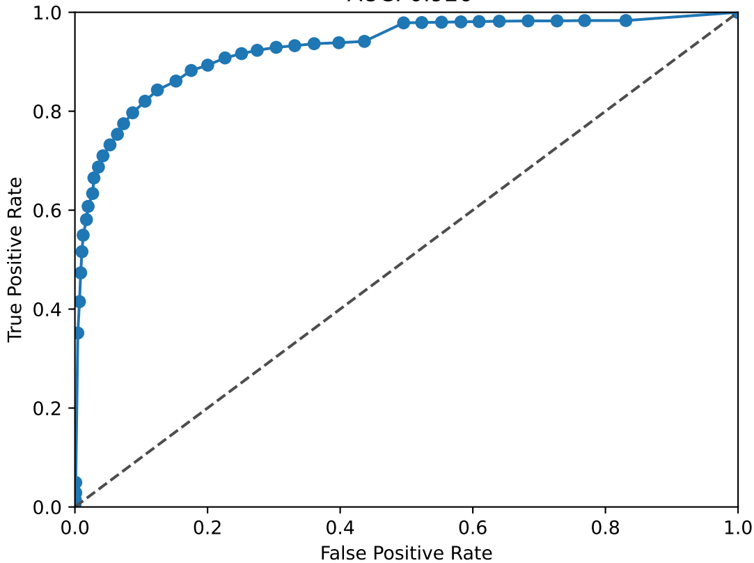
STAT2 ROC Curve AUC: 0.926
