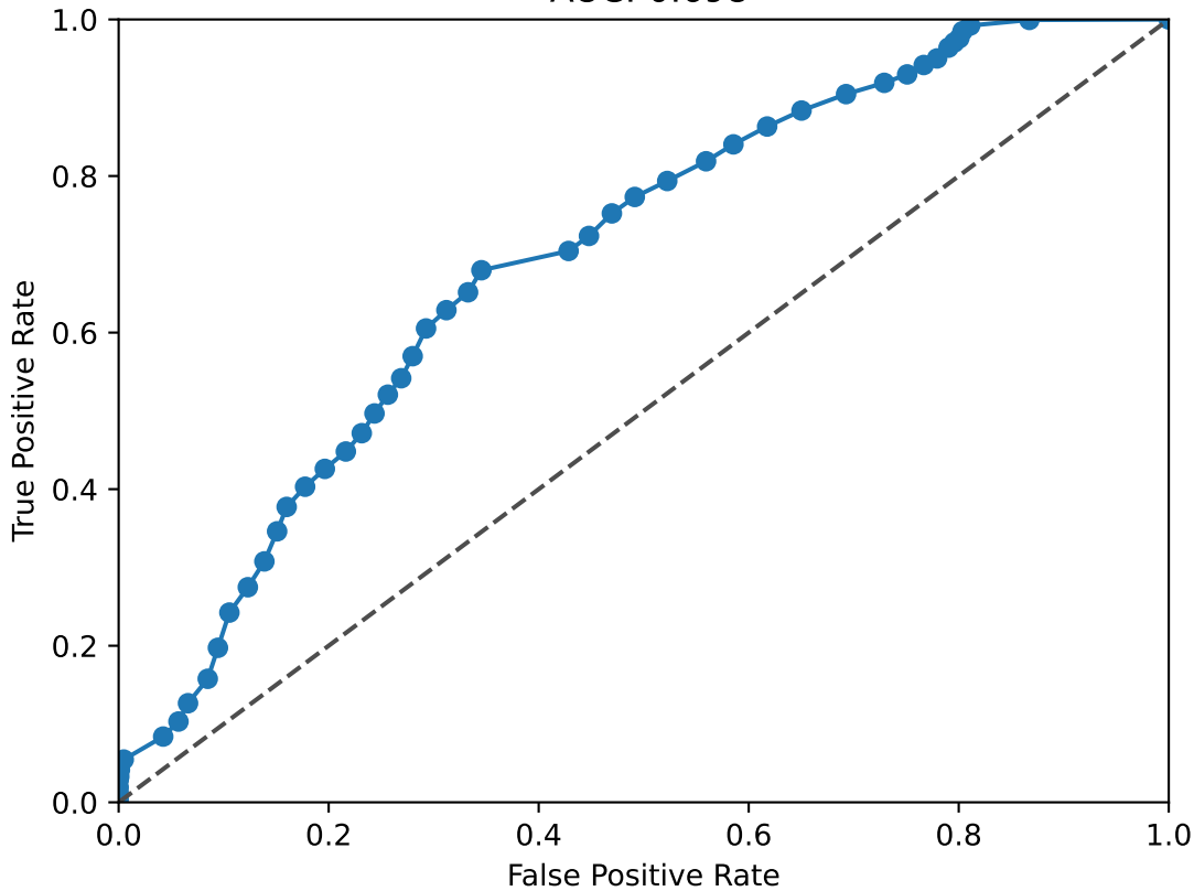
ASCL1 ROC Curve AUC: 0.698
