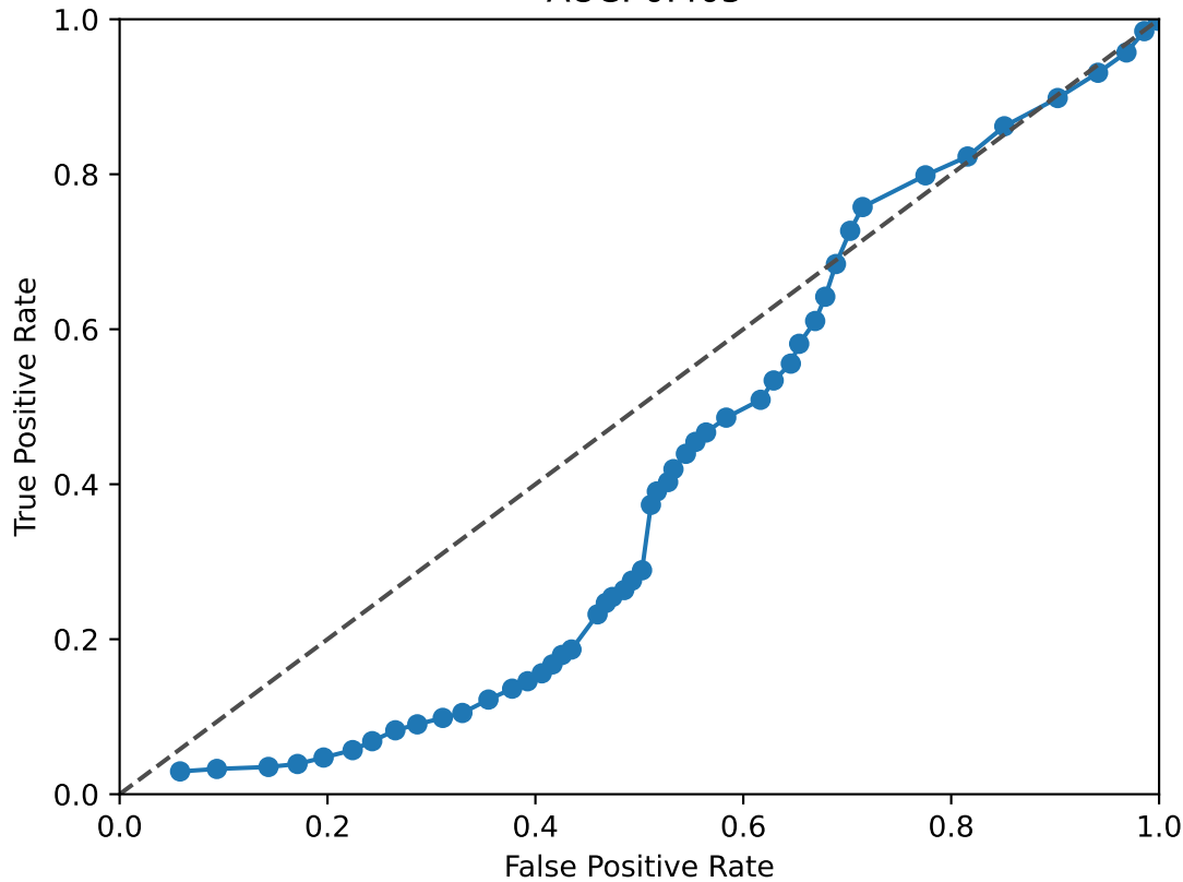
ETS1 ROC Curve AUC: 0.405
