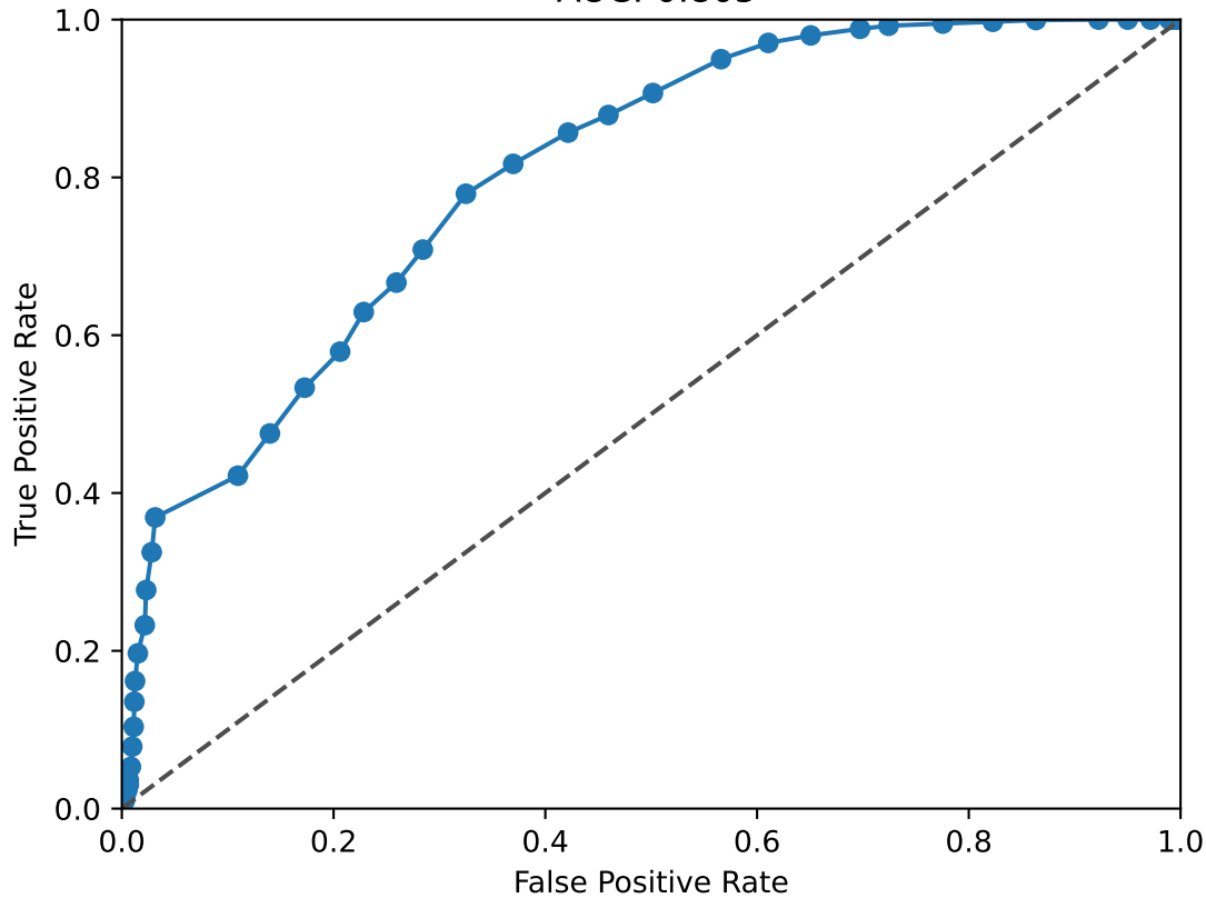
FOS ROC Curve AUC: 0.805
