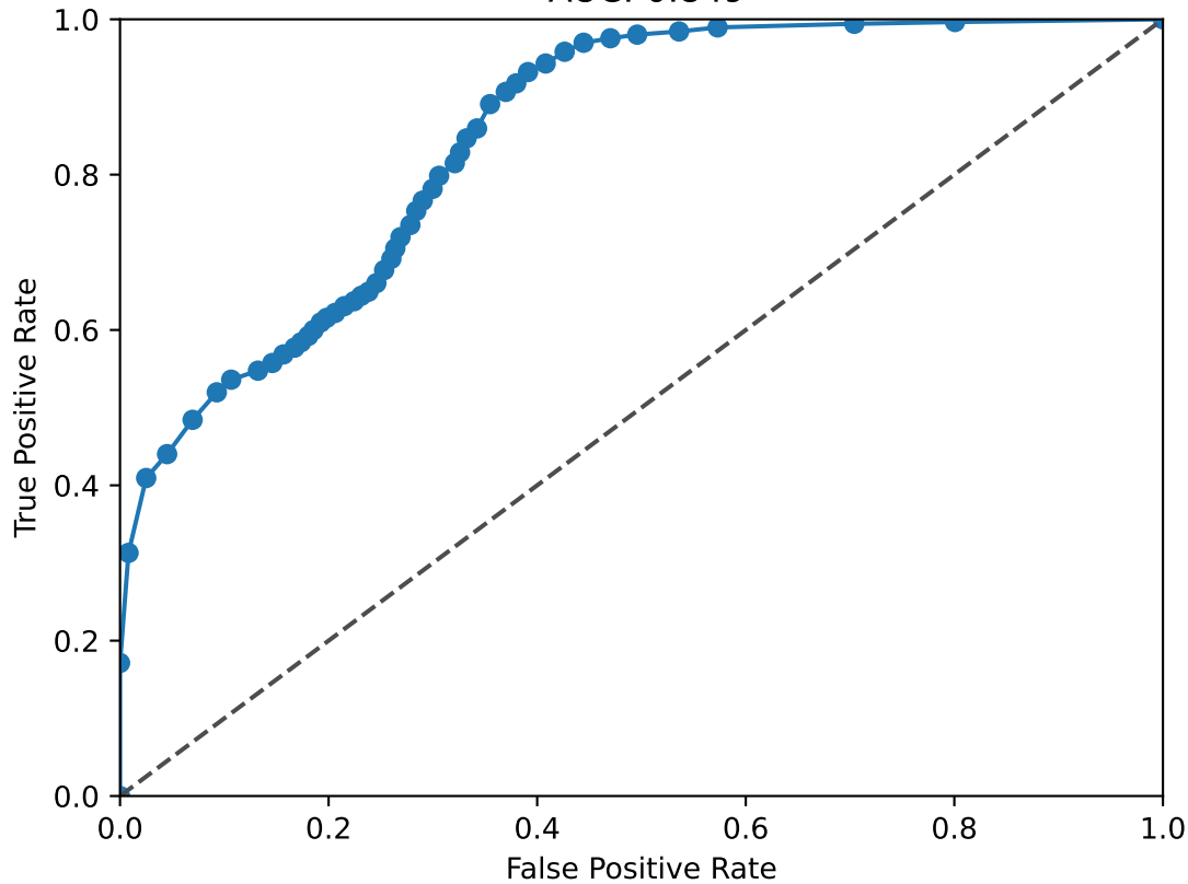
GRHL2 ROC Curve AUC: 0.849
