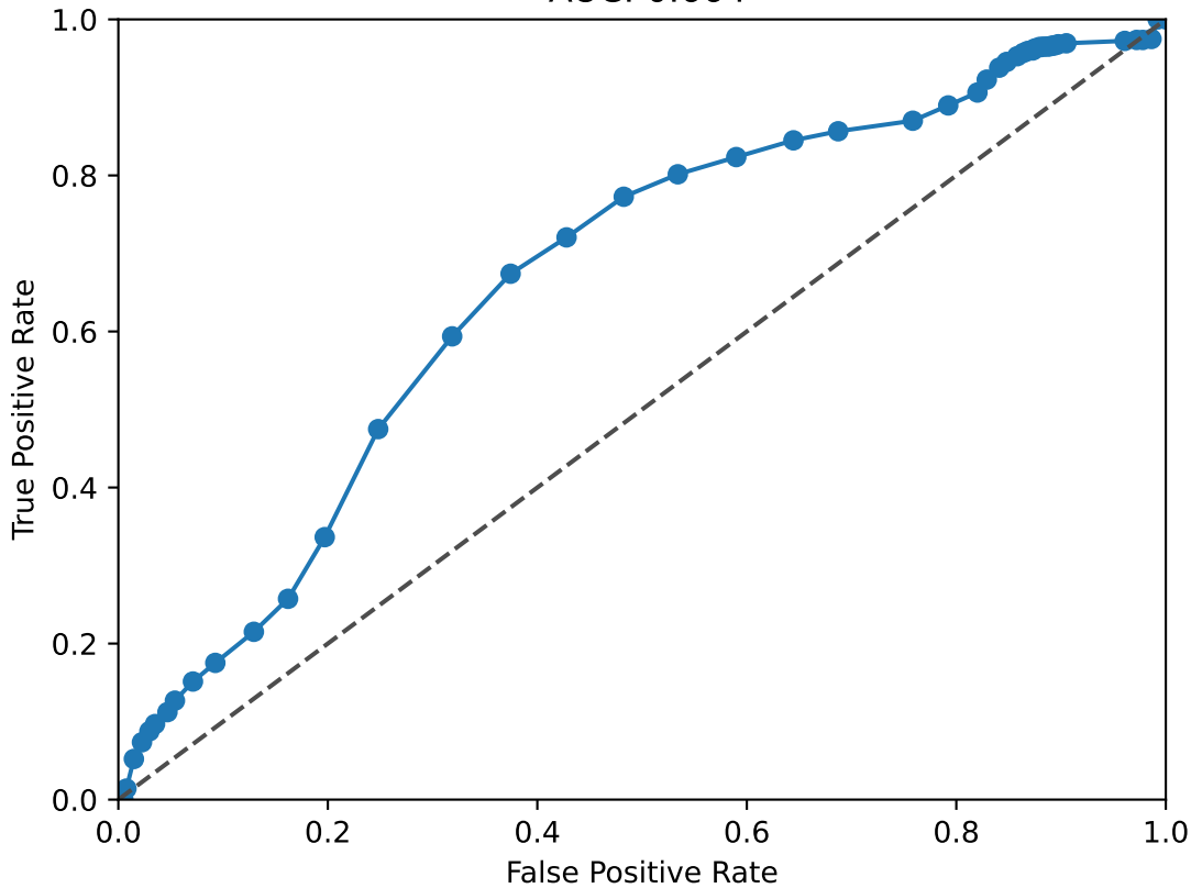
KMT2A ROC Curve AUC: 0.664
