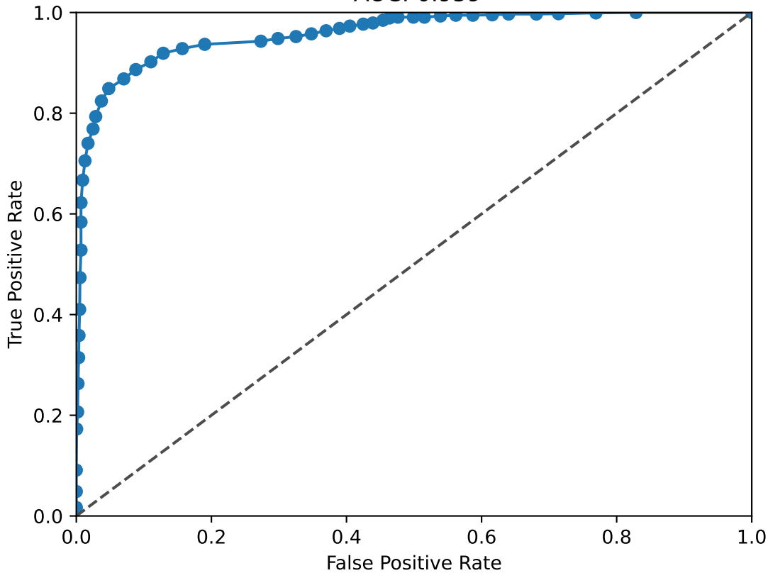
NFIA ROC Curve AUC: 0.959
