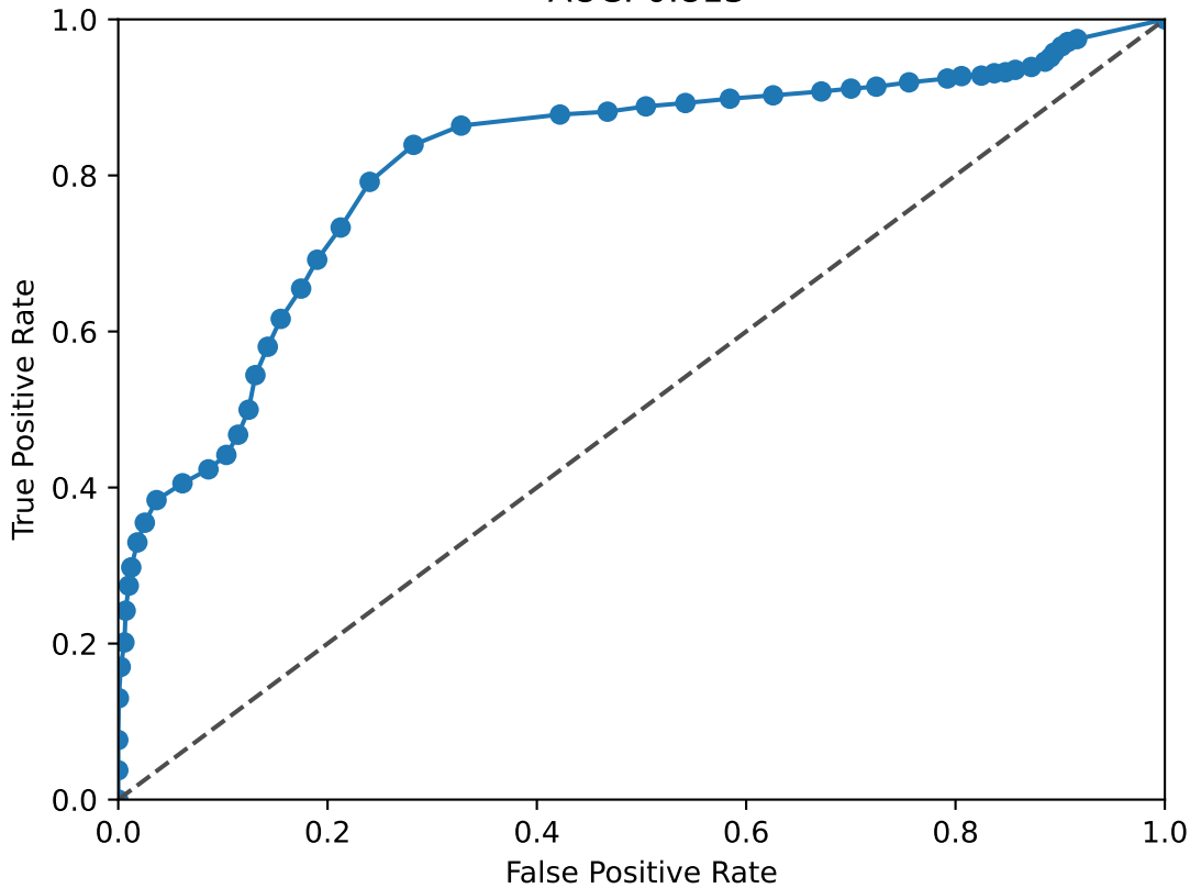
NFIB ROC Curve AUC: 0.813
