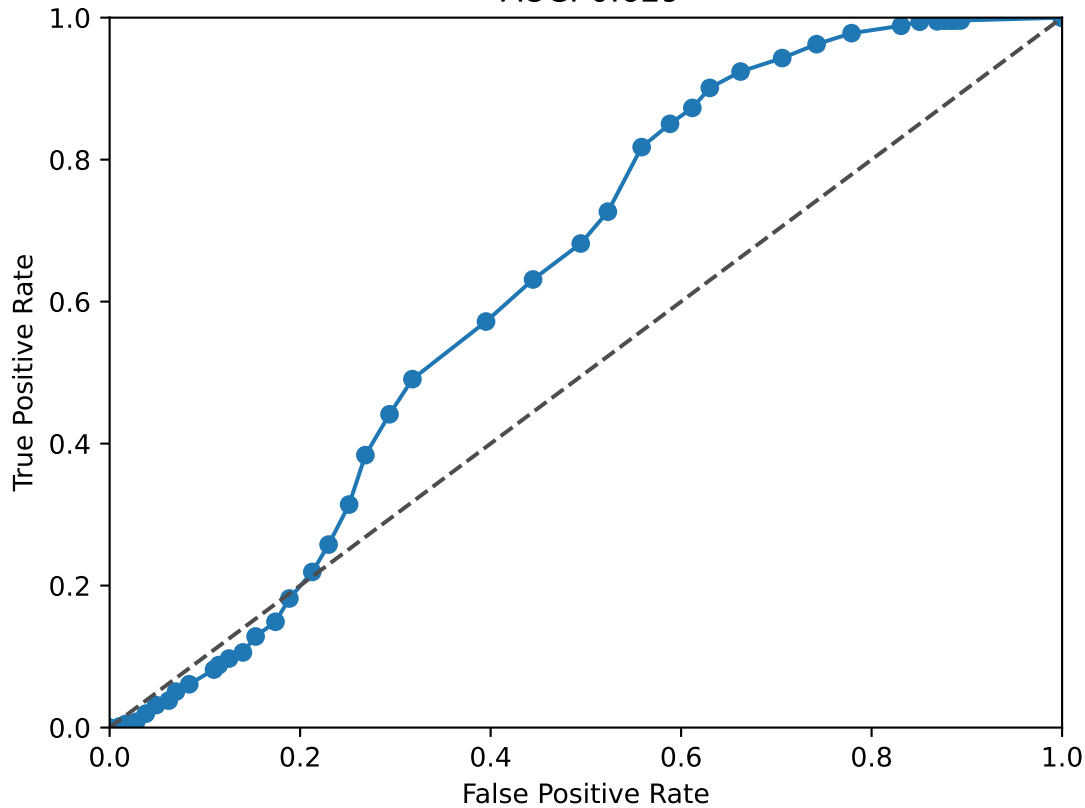
PBX1 ROC Curve AUC: 0.629
