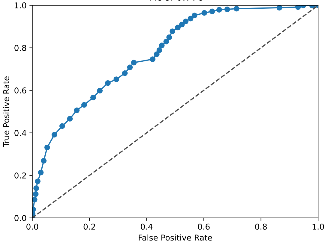
PKNOX2 ROC Curve AUC: 0.778
