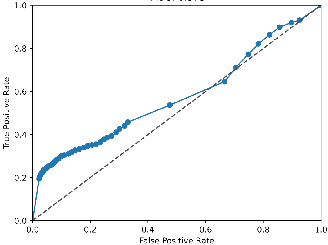
PROX1 ROC Curve AUC: 0.575
