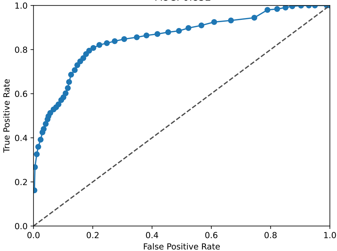
RORA_RORB ROC Curve AUC: 0.852
