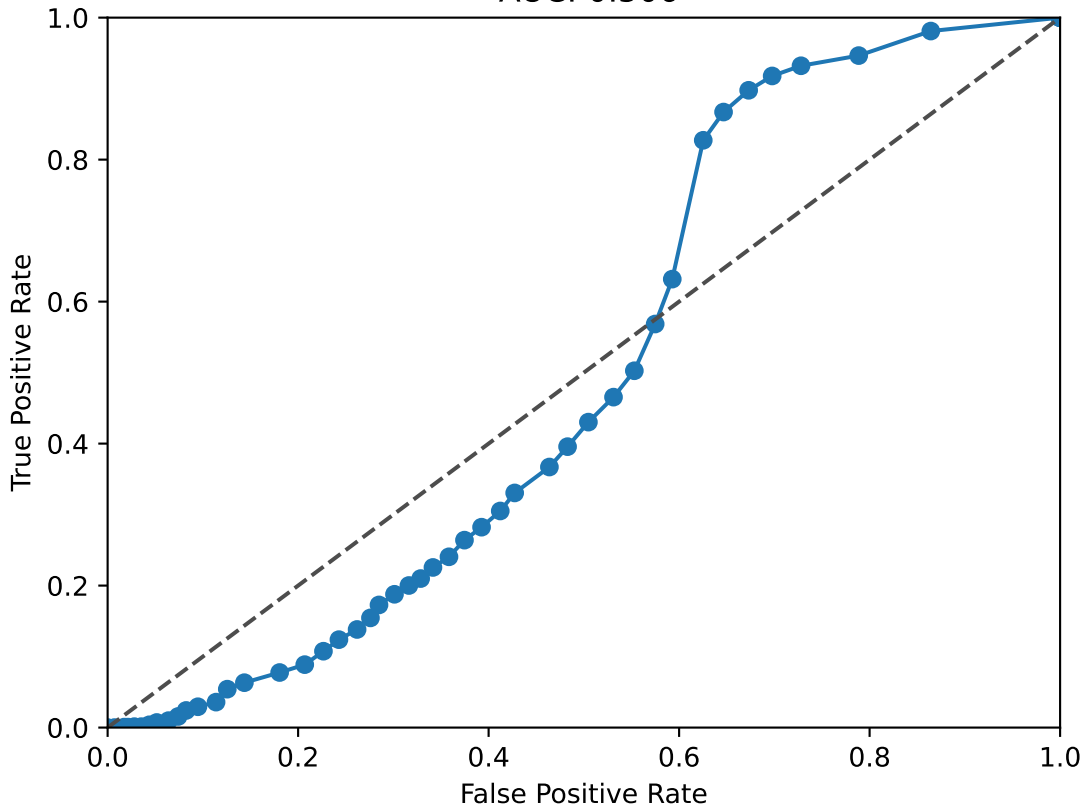
SOX11 ROC Curve AUC: 0.506
