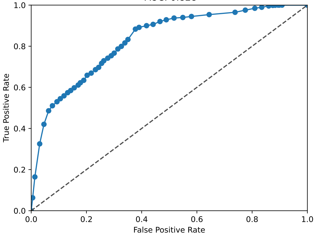
TEAD1 ROC Curve AUC: 0.828
