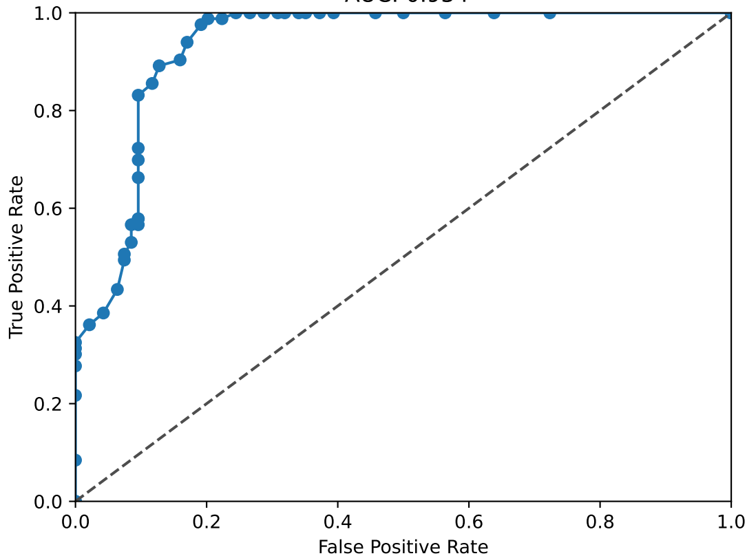
EGR1 ROC Curve AUC: 0.934
