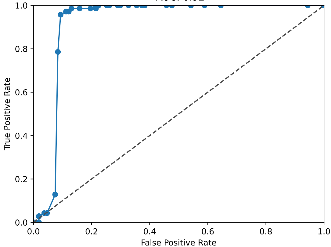
EPCAM ROC Curve AUC: 0.92
