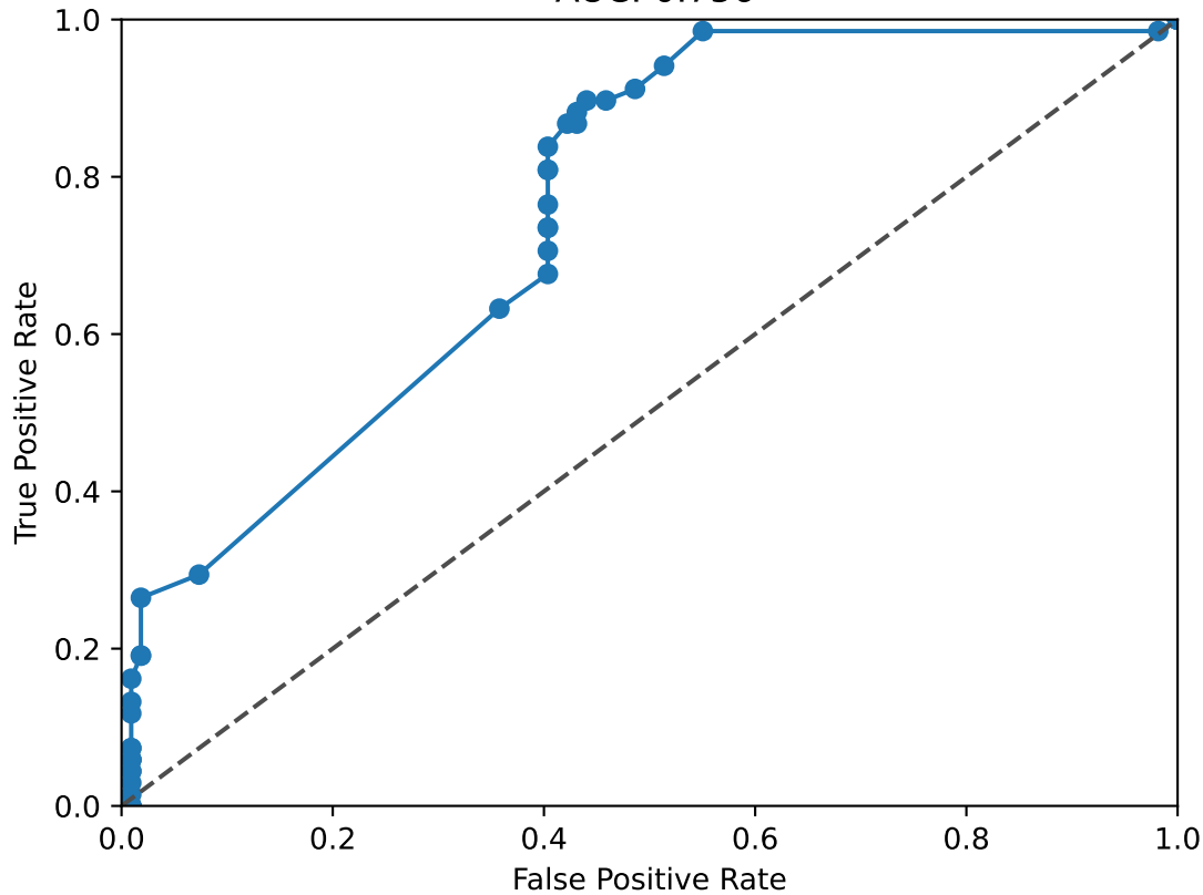
ETS1 ROC Curve AUC: 0.756
