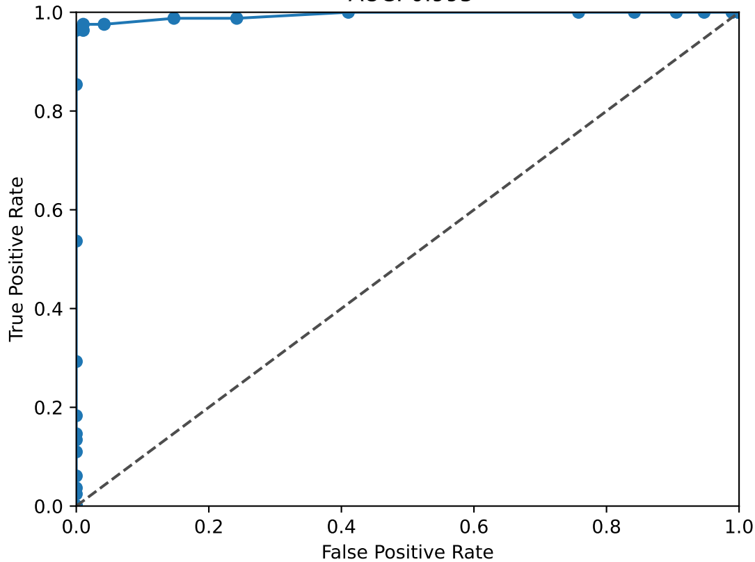
FOS ROC Curve AUC: 0.995
