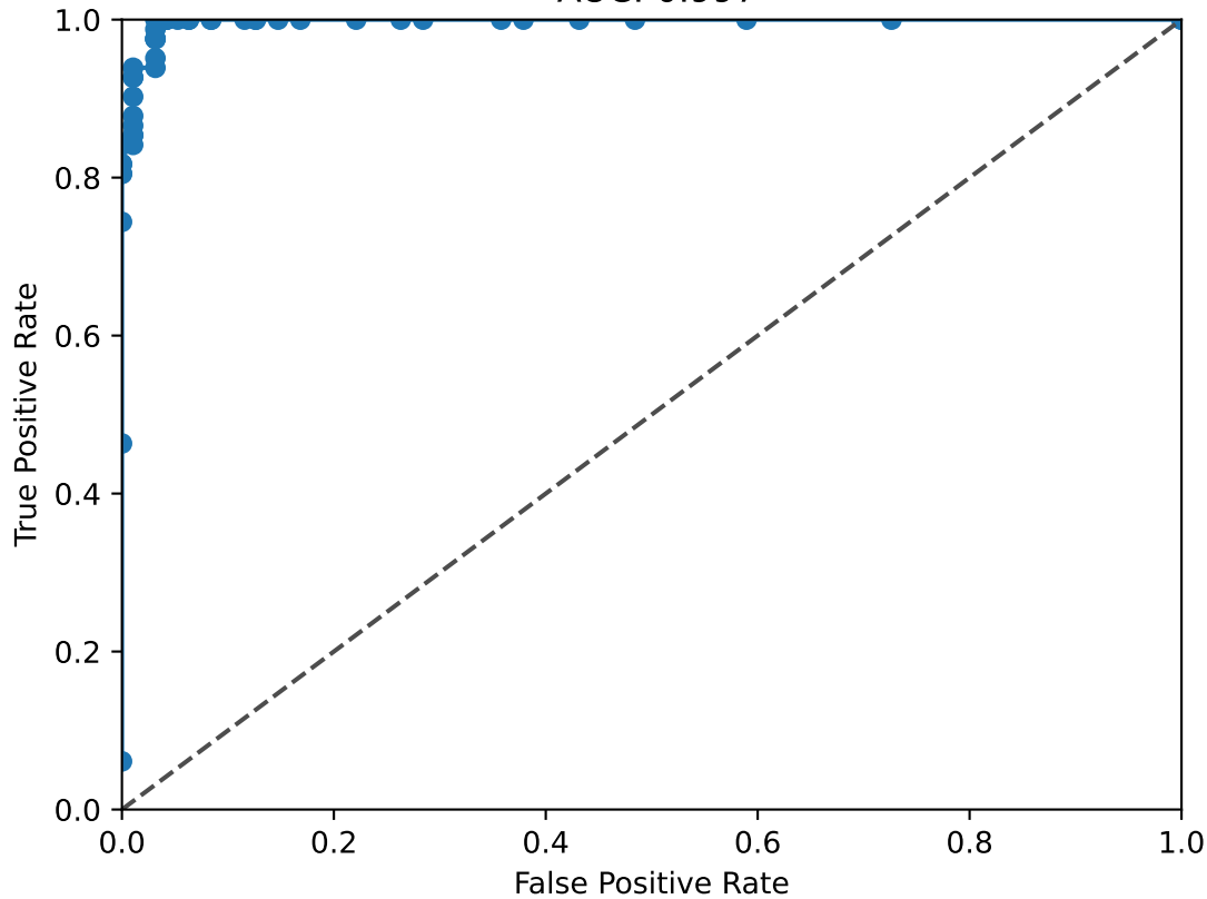
HSF2 ROC Curve AUC: 0.997
