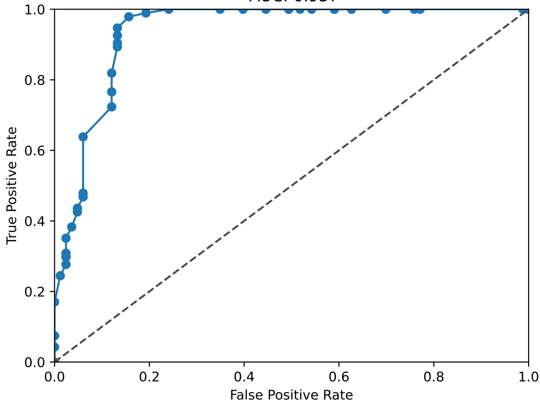
NFATC2 ROC Curve AUC: 0.937
