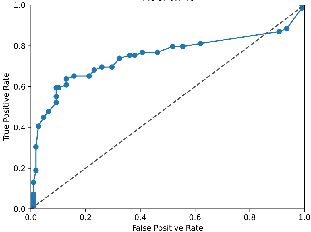
PKNOX2 ROC Curve AUC: 0.746
