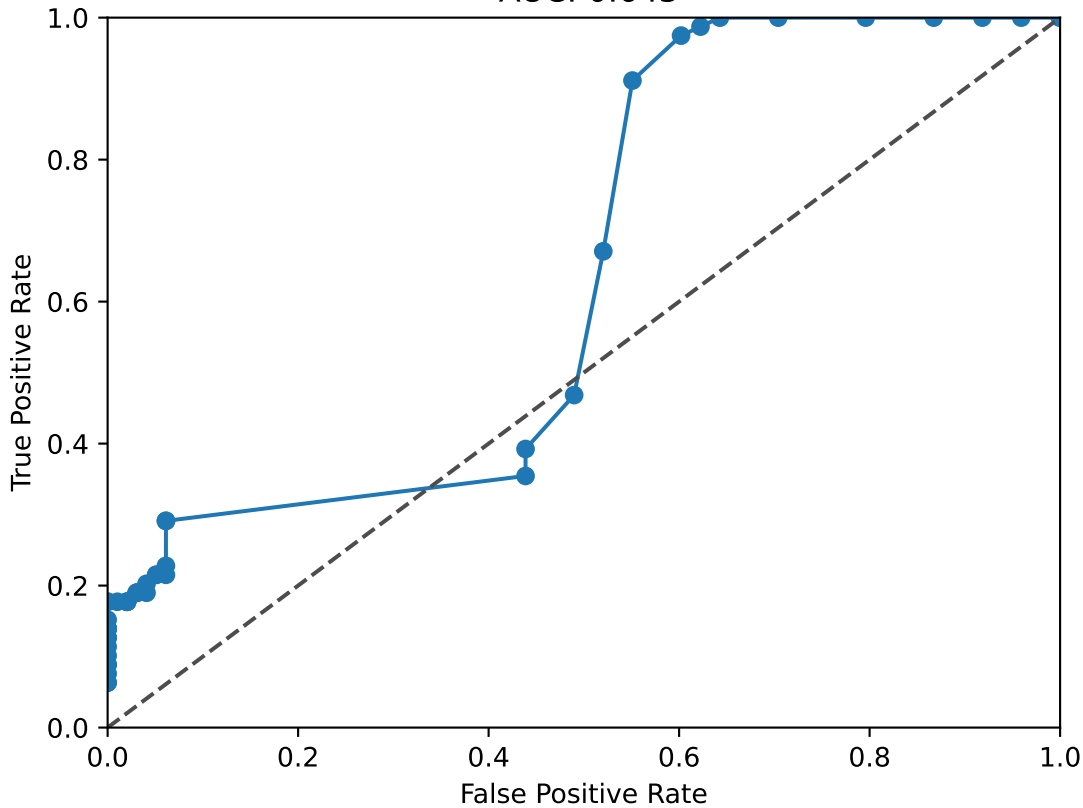
REST ROC Curve AUC: 0.643
