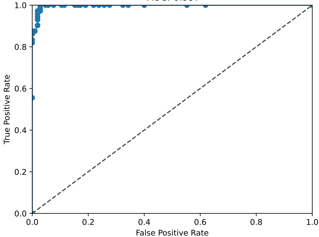
TEAD1 ROC Curve AUC: 0.997
