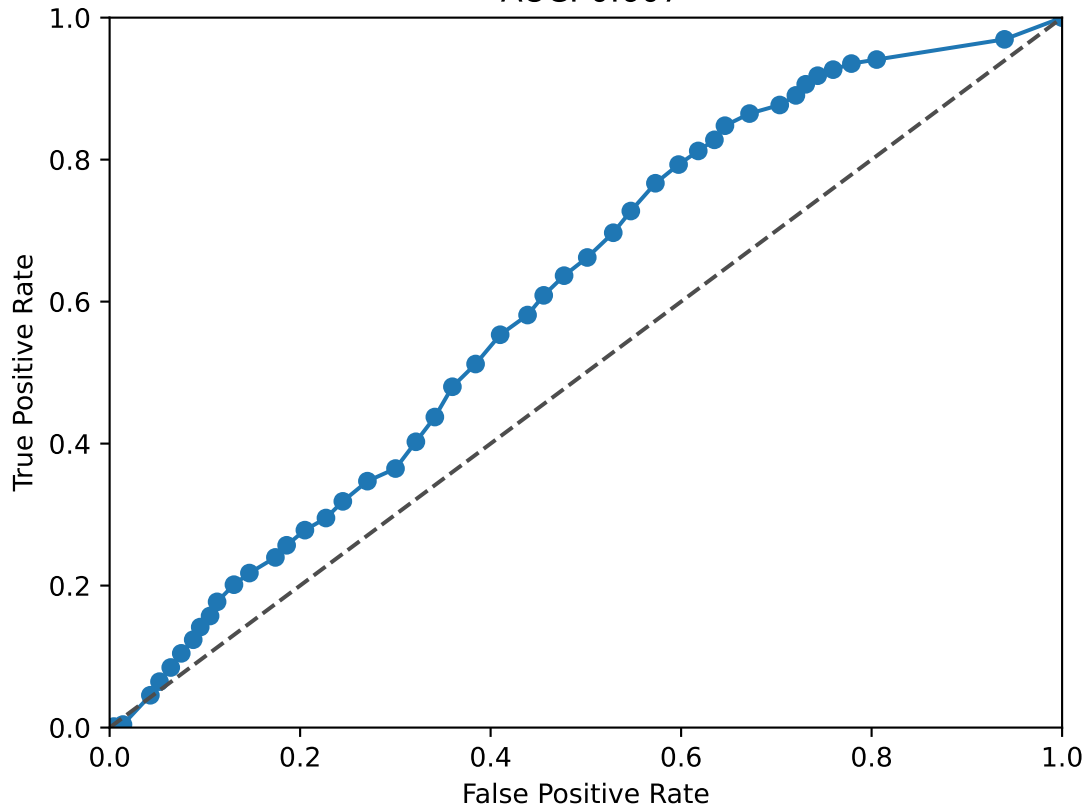
ASCL1 ROC Curve AUC: 0.607
