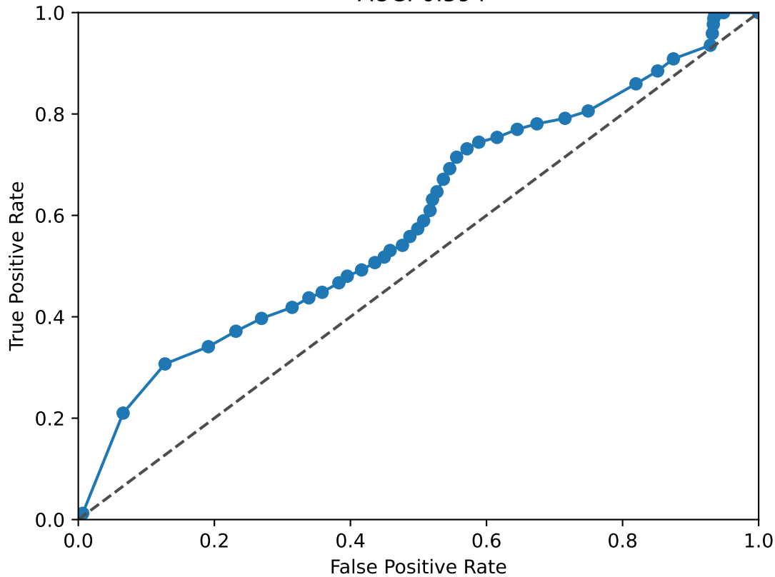
BACH1 ROC Curve AUC: 0.594
