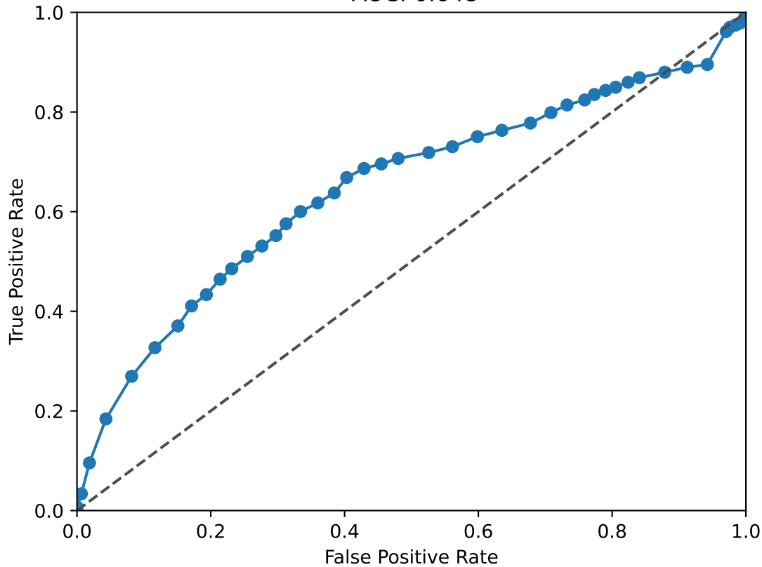
CUX2 ROC Curve AUC: 0.648
