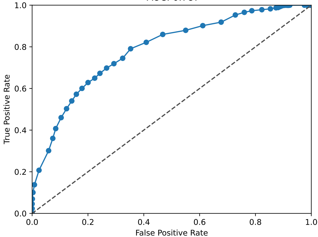
EGR1 ROC Curve AUC: 0.787
