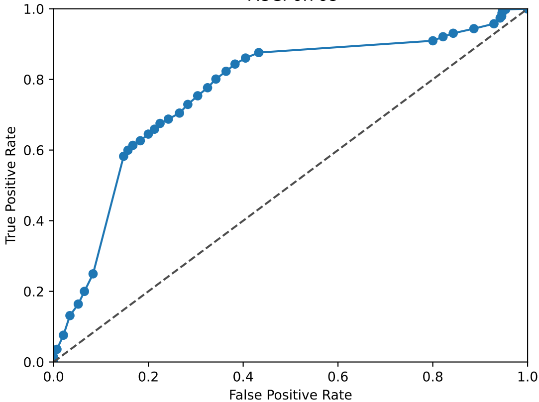
EHF ROC Curve AUC: 0.768
