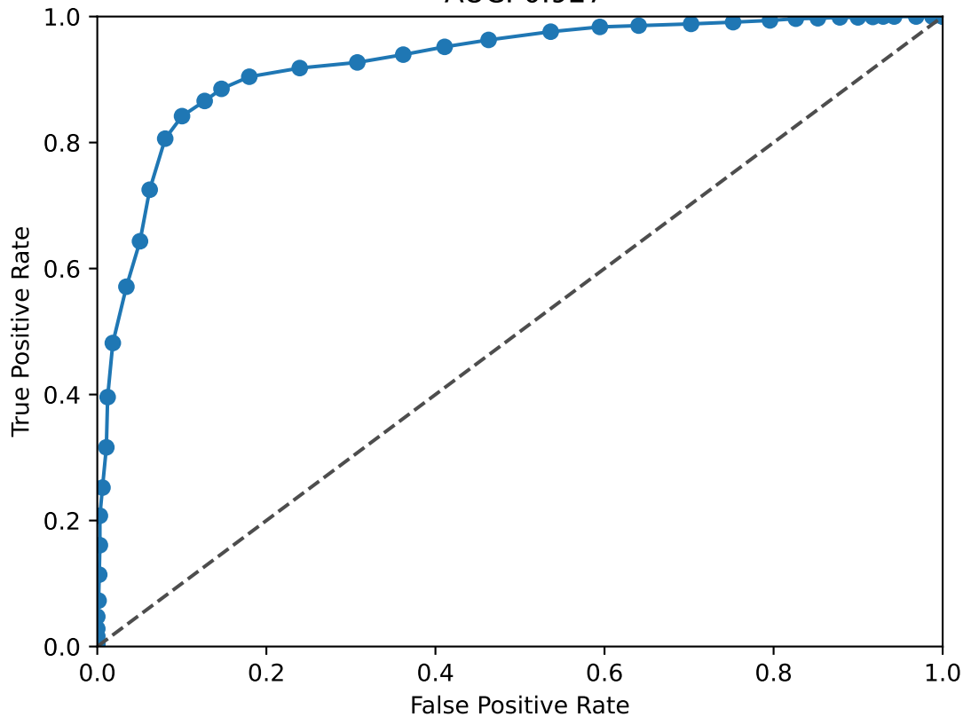
FOS ROC Curve AUC: 0.927
