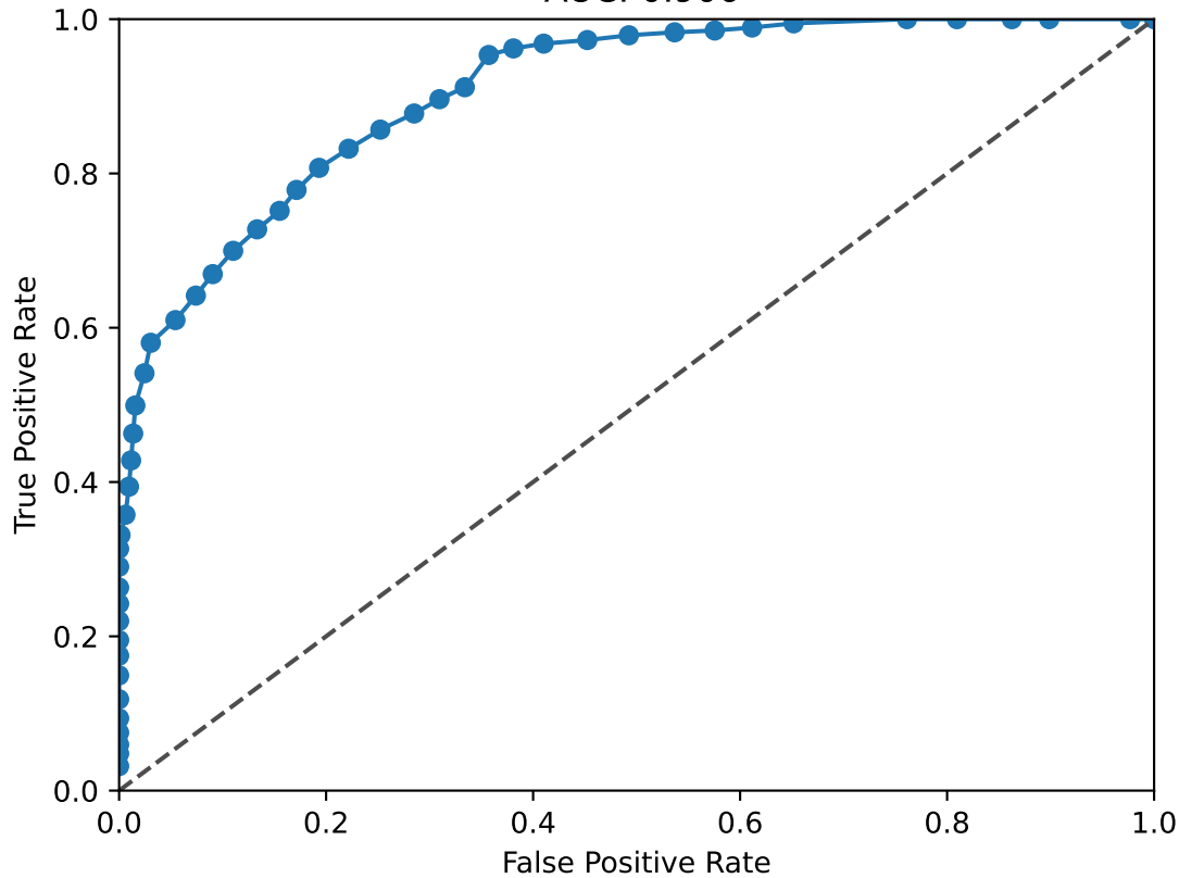
HSF2 ROC Curve AUC: 0.906
