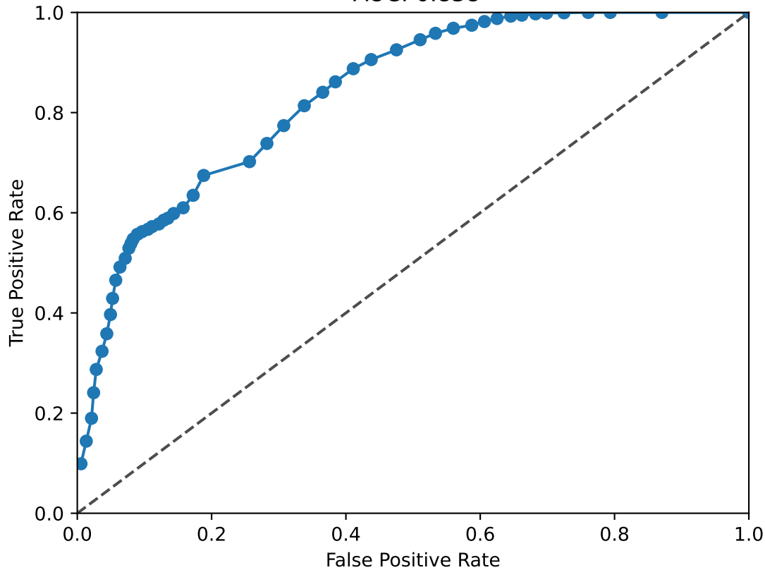
JUN ROC Curve AUC: 0.838
