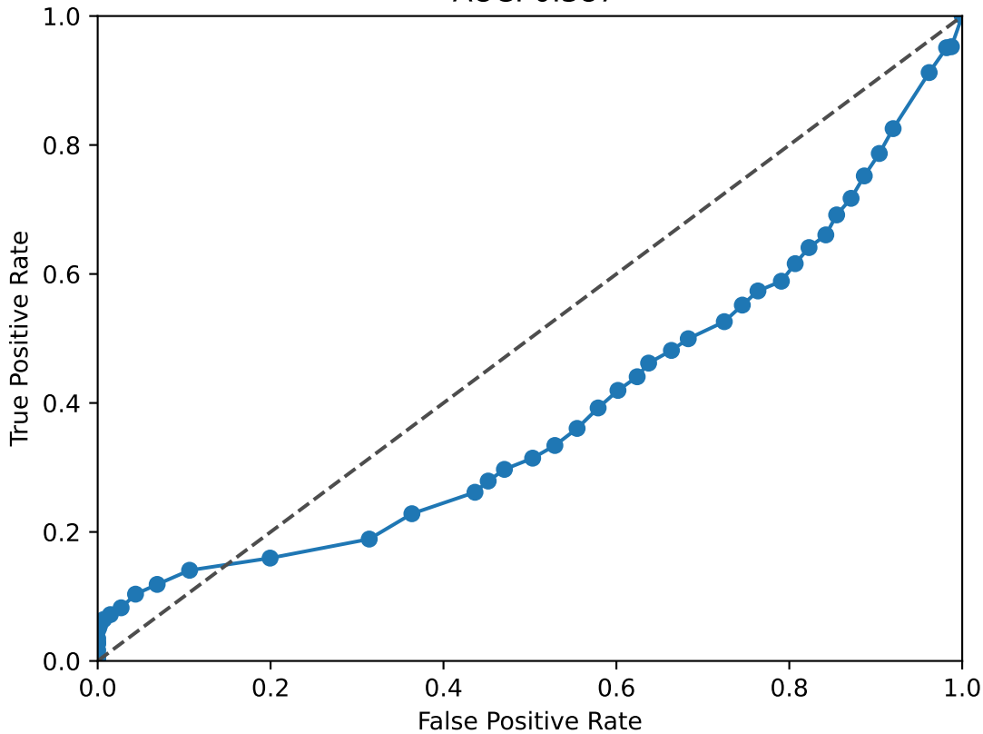
NFIA ROC Curve AUC: 0.387
