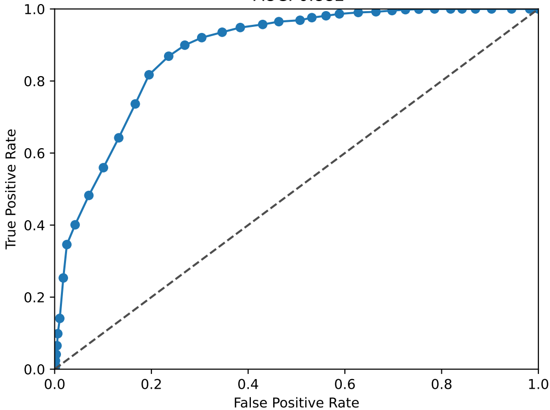
NFIB ROC Curve AUC: 0.882
