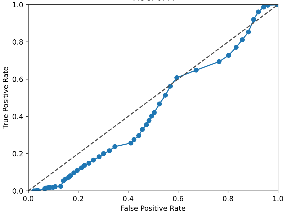
NFIX ROC Curve AUC: 0.44
