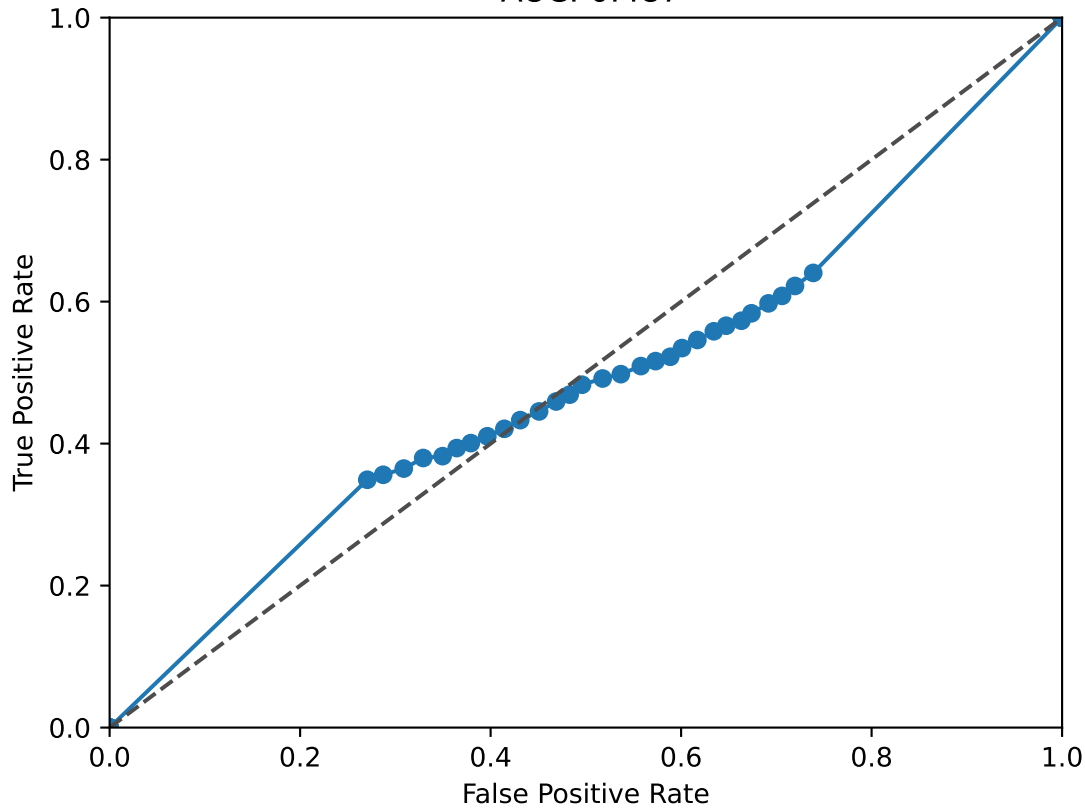
THRB ROC Curve AUC: 0.487
