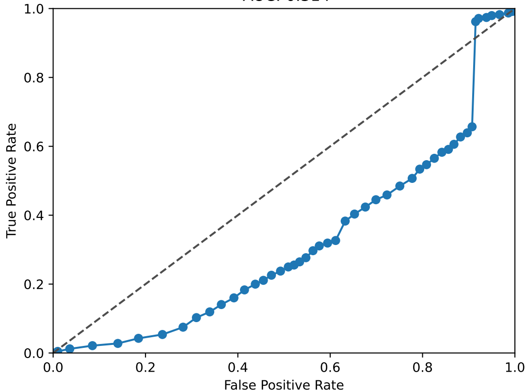
CUX2 ROC Curve AUC: 0.314
