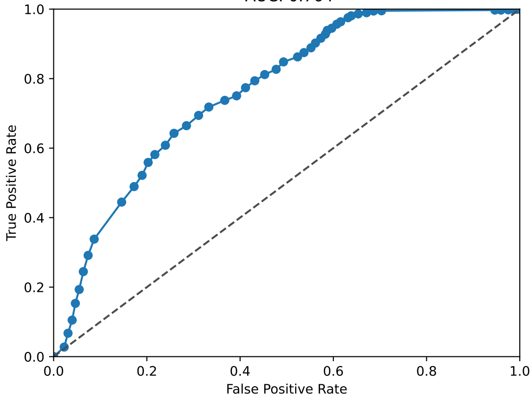
EGR1 ROC Curve AUC: 0.764
