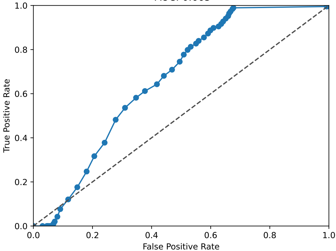
EPCAM ROC Curve AUC: 0.663
