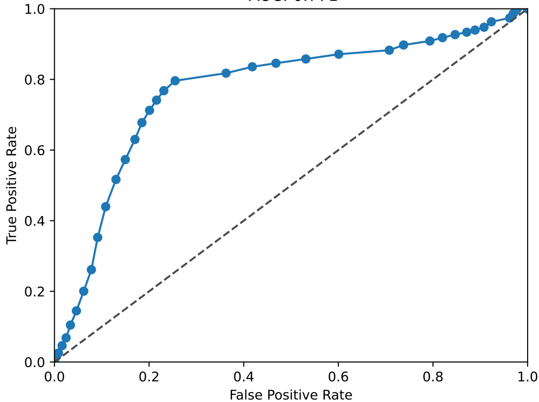
FOS ROC Curve AUC: 0.771
