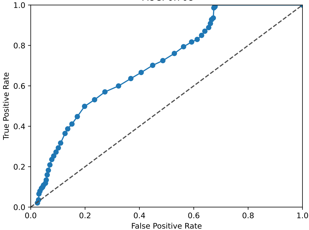
HES1 ROC Curve AUC: 0.708
