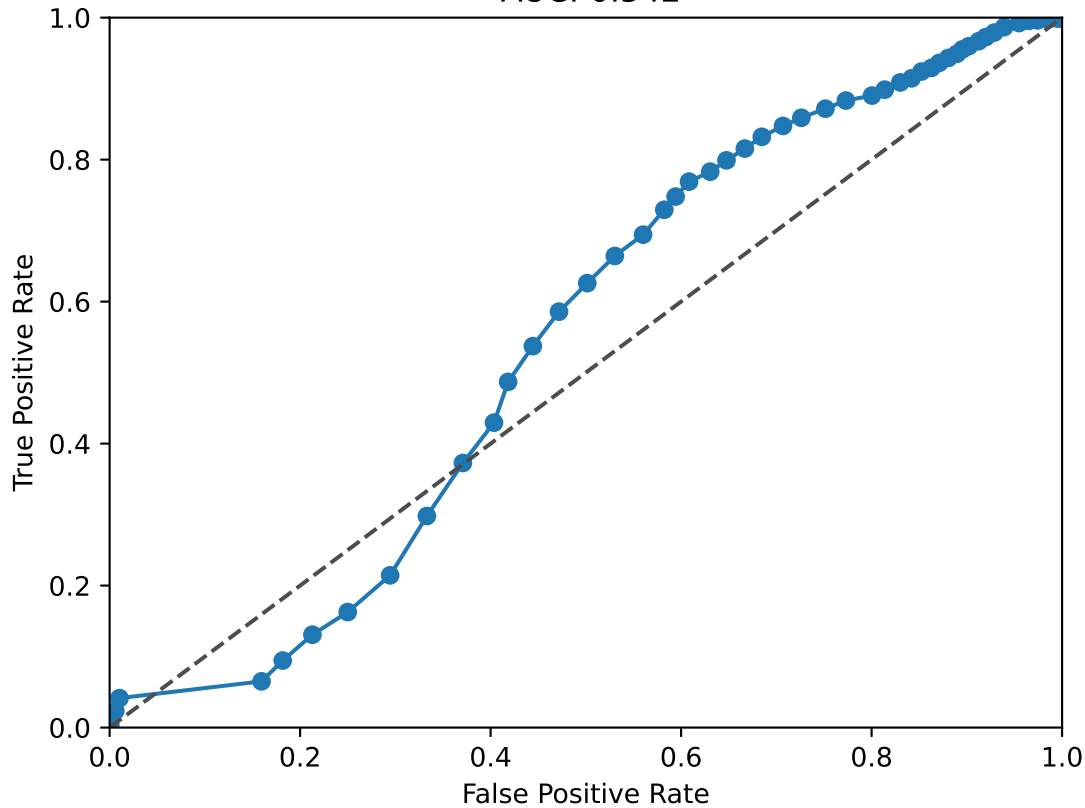
KMT2A ROC Curve AUC: 0.542
