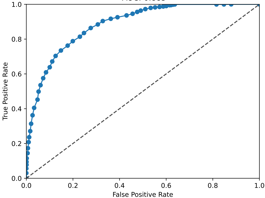
NFIB ROC Curve AUC: 0.885
