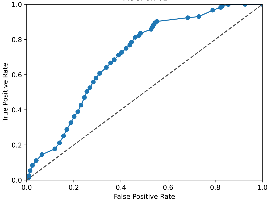
PKNOX2 ROC Curve AUC: 0.702
