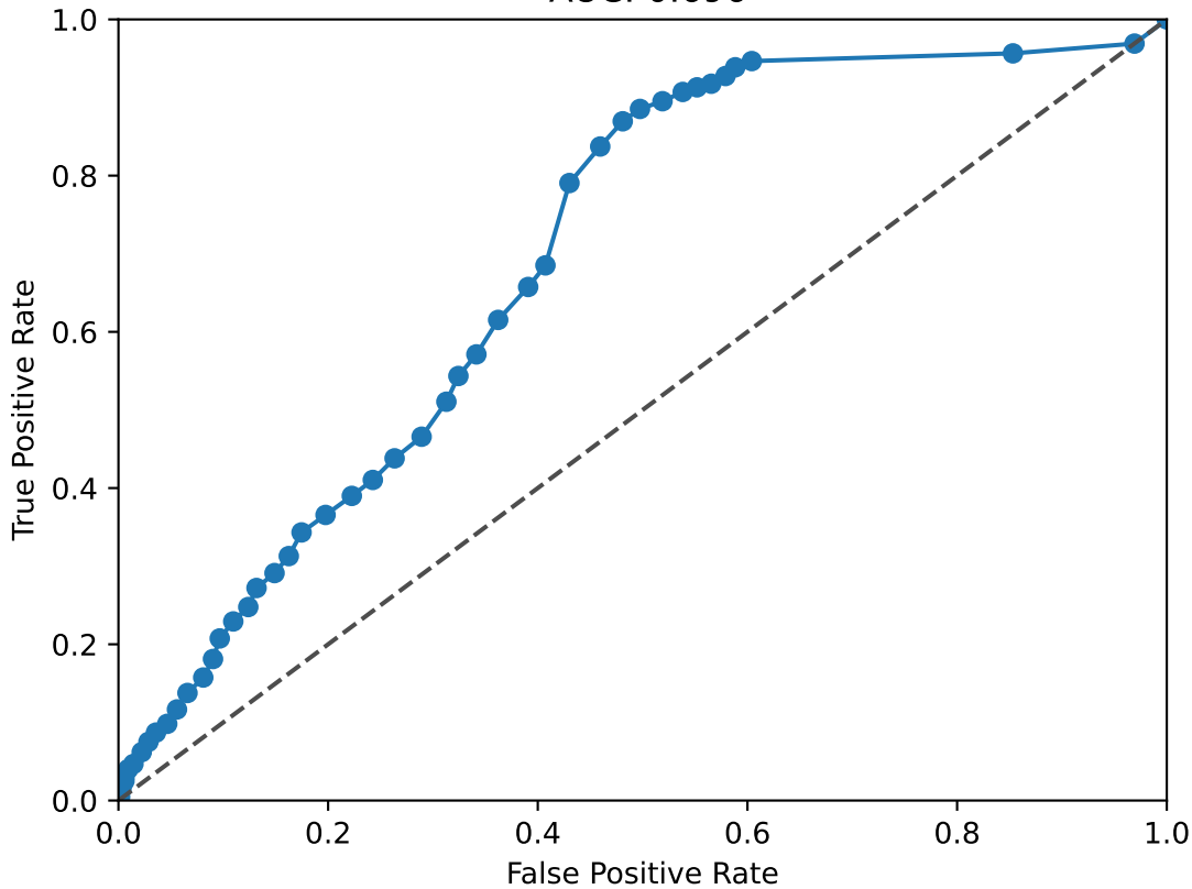
SIX1 ROC Curve AUC: 0.696
