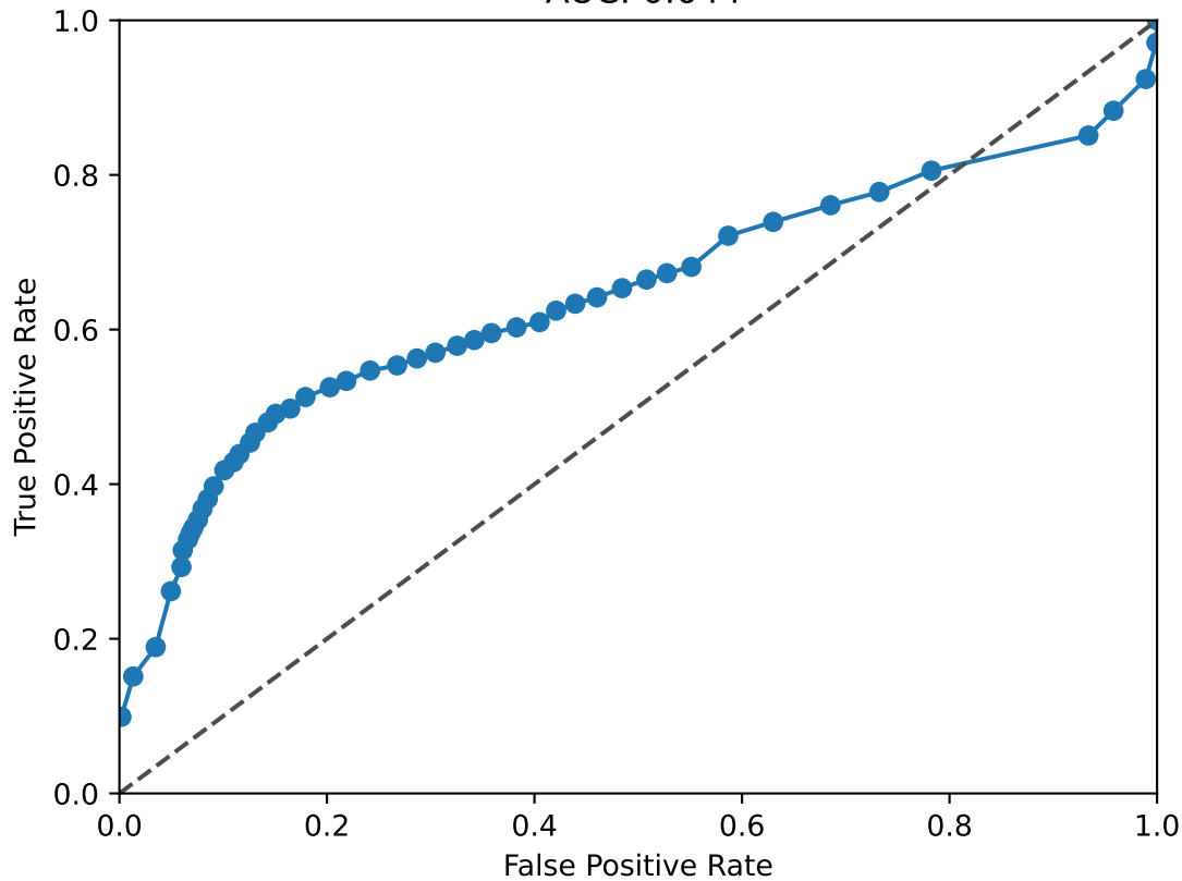
SMAD3 ROC Curve AUC: 0.644
