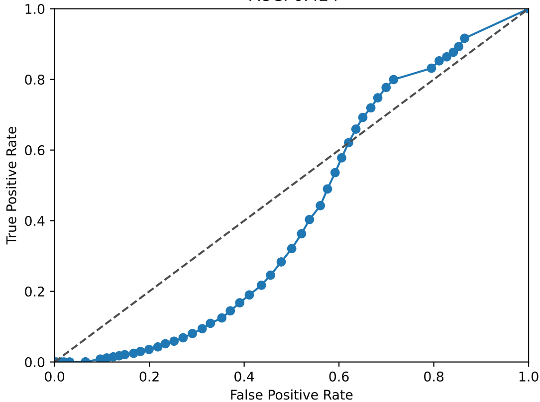
ASCL1 ROC Curve AUC: 0.424
