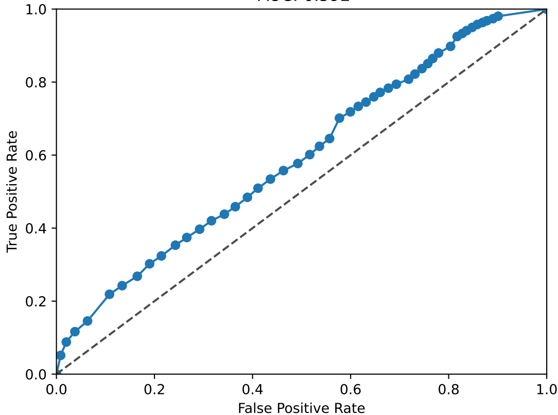
BACH1 ROC Curve AUC: 0.592
